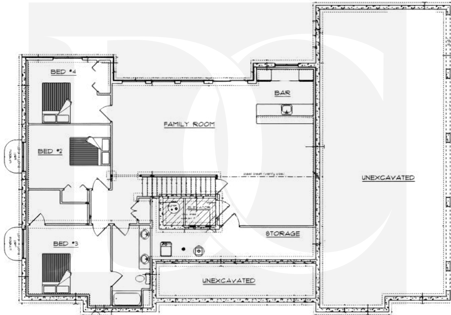
1430 SQ FT FINISHED BASEMENT
