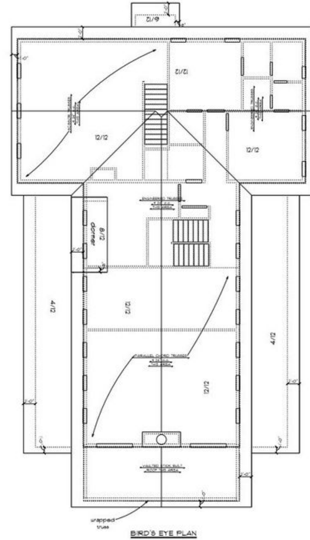
BIRD'S EYE PLAN
