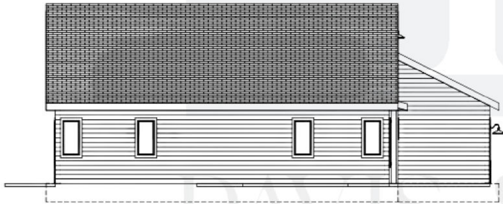
Back and Side Elevation
