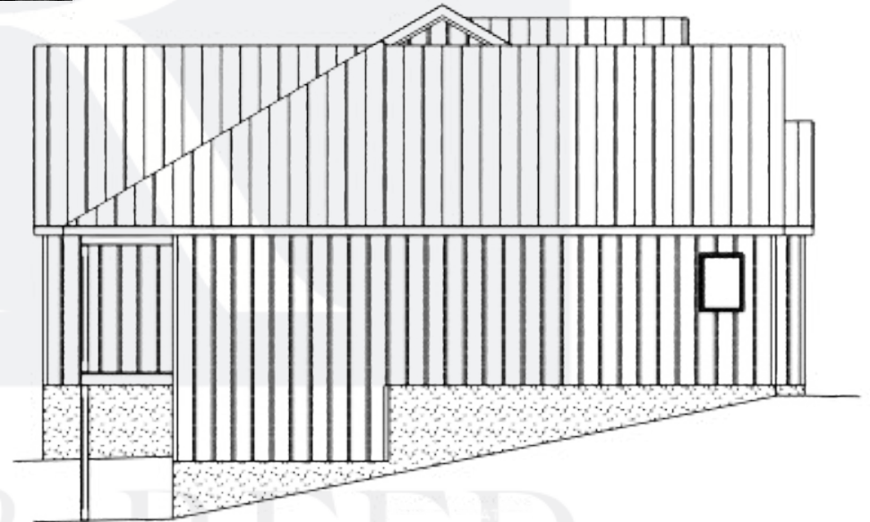
Left and Right Elevations
